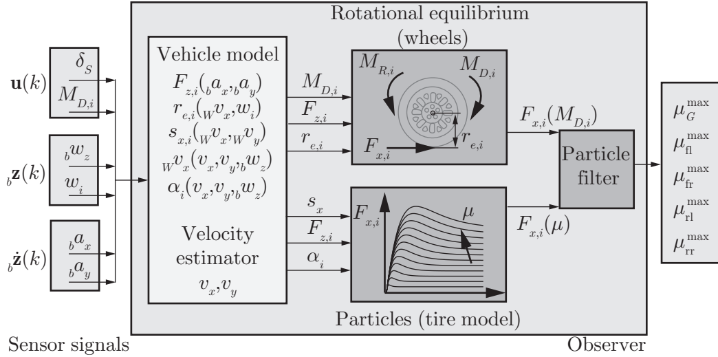
Figure 5.4.: Schematic structure of tire/road friction estimator showing the driver's inputs \mathbf{u}(k) , the measurement inputs \mathbf{z}(k) and \dot{\mathbf{z}}(k) on the left side and the estimation outputs \hat{\mathbf{x}}(k) comprising \mu_G^{\max}(k) and \mu_i^{\max}(k) on the right side. The observer model consists of the vehicle model (cf. Section 3.2) and the velocity estimator, which deliver the inputs needed to calculate the expected F_{x,i} based on the wheel's angular momentum and the tire forces from the horizontal tire model for N particles of \mu^{\max} , which are then forwarded to the particle filter.
