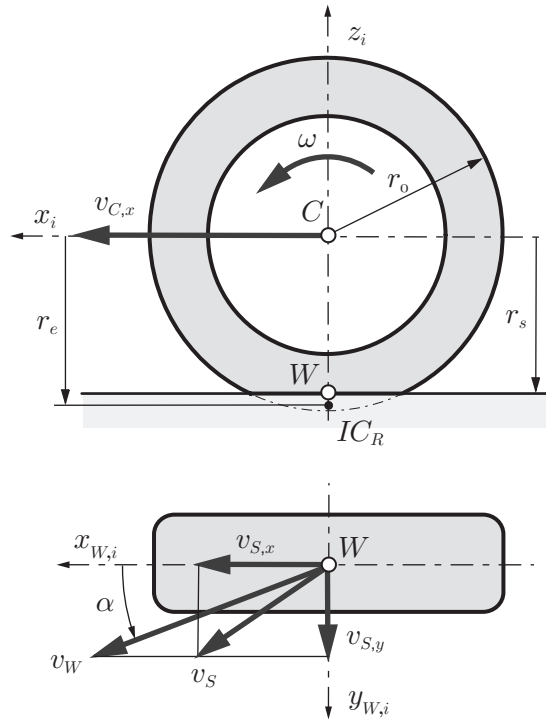
Figure 2.2.: Kinematic wheel quantities of the i -th wheel coordinate system \{\mathcal{O}_i, x_i, y_i, z_i\} with its origin in the wheel centre C according to ISO 8855 , [fSI11]; the graphic depiction is based on Hirschberg , [HW12, p.16]. The velocity in the contact point W between tire and road is described by its components v_{W,x} and v_{W,y} . The components v_{S,x} and v_{S,y} of the sliding velocity v_S differ from v_W by \omega \cdot r_e . The effective tire radius r_e is the distance between the wheel centre C and the instantaneous centre of rotation IC_R . In addition, the unloaded tire radius r_0 , the static tire radius r_s , the wheel speed \omega and the lateral slip angle \alpha are shown.
