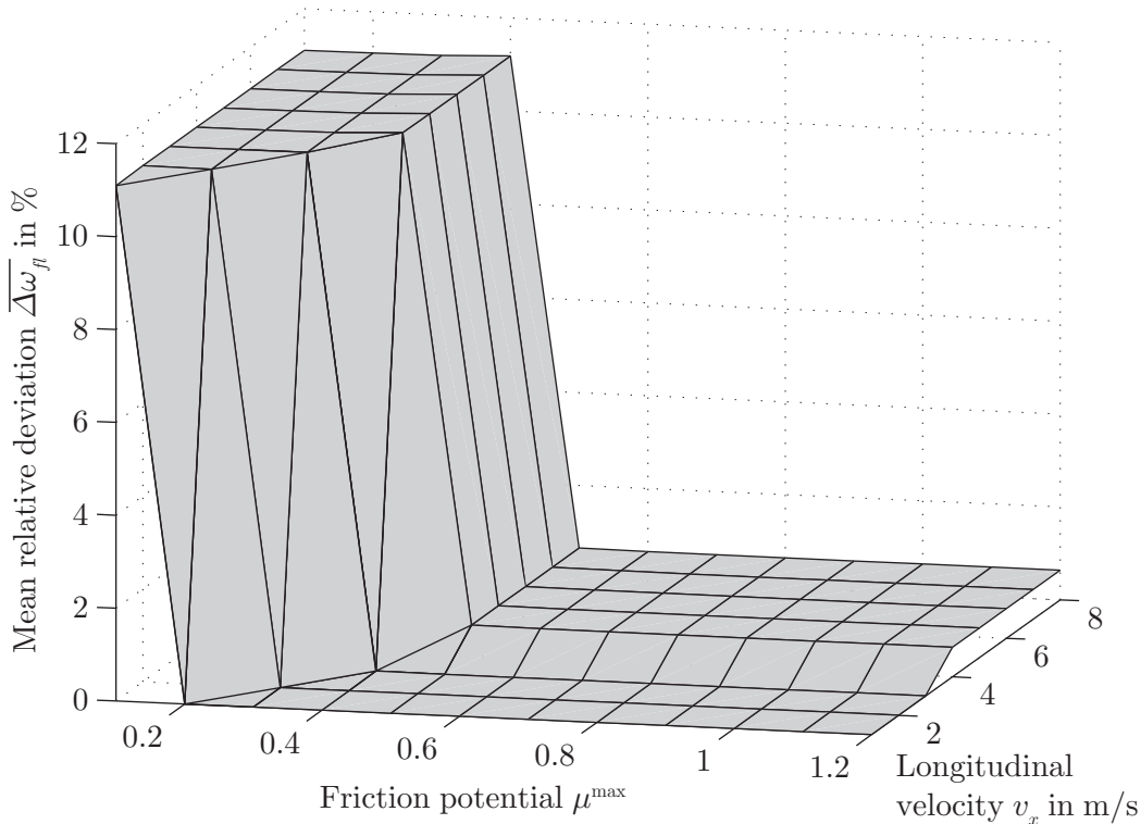
Figure 3.4.: Mean relative deviation \overline{\Delta\omega_{fl}} of the front left wheel’s rotational speed during an accelerating manoeuvre with varied wheel moment of inertia. It can be seen that for low \mu^{\max} \leq 0.5 , there is an abrupt change in the characteristics. This occurs as the front wheels start to spin in order to be able to follow the given speed profile. The variation of the moment of inertia results in different wheel rotational accelerations that influence \overline{\Delta\omega_{fl}} as shown.
