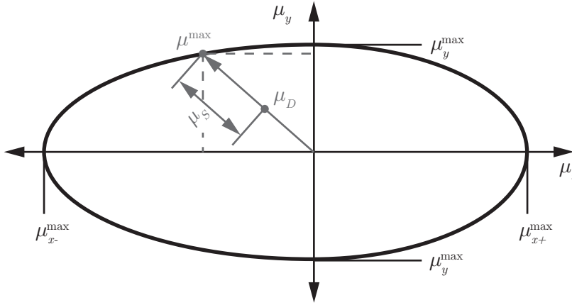
Figure 2.5.: Schematic representation of the combined friction potential based on the outer limits of a Krempel diagram, based on Heißing et al. , [HE11, p.62]. The absolute value of \mu_{x-}^{\max} is higher than that of \mu_{x+}^{\max} when considering the vehicle's different braking, acceleration and cornering capabilities.
