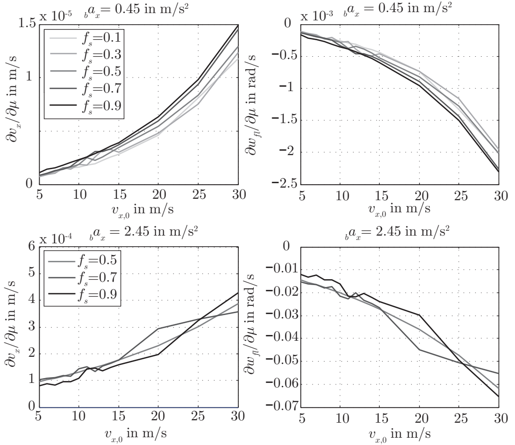
Figure 4.4.: Dependence of selected sensitivities \partial v_x/\partial\mu ( left ) and \partial\omega_{fl}/\partial\mu ( right ) versus the initial longitudinal velocity v_{x,0} for \mu^{\max} = 1 for pure longitudinal acceleration of 0.45 \text{ m/s}^2 ( above ) and 2.45 \text{ m/s}^2 ( below ) and different scaling factors f_s within the simulation.
