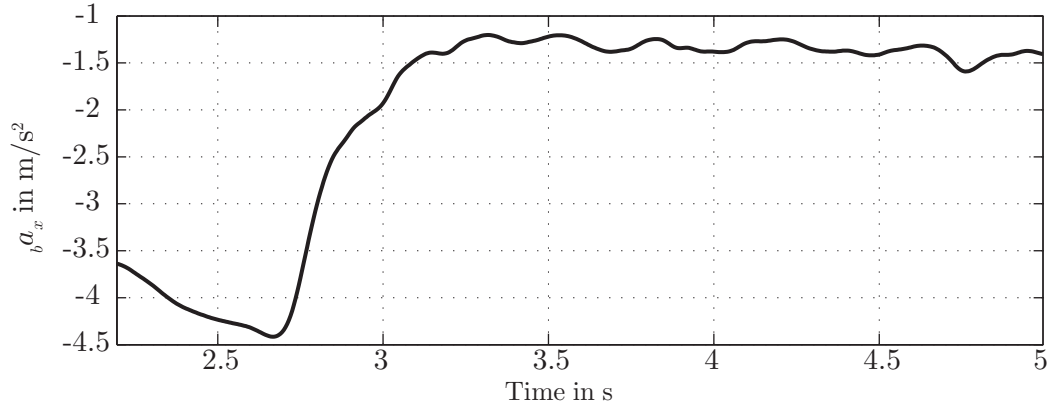
Figure 6.7.: Longitudinal acceleration {}_b a_x during a braking manoeuvre on varying \mu^{\max} with a maximum deceleration {}_b a_x \approx -4.5 m/s 2 . The manoeuvre was started at v_x \approx 50 km/h and ended at 30 km/h.
