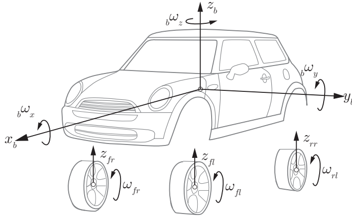
Figure 3.1.: Degrees of freedom (DOF) of vehicle model used for model complexity evaluation. The DOF include the vehicle's body translational \{x_b, y_b, z_b\} and rotational \{{}^b\omega_x, {}^b\omega_y, {}^b\omega_z\} degrees of freedom, as well as the wheels' vertical displacements \{z_{fl}, z_{fr}, z_{rl}, z_{rr}\} and the wheel rotational speeds \{\omega_{fl}, \omega_{fr}, \omega_{rl}, \omega_{rr}\} , with the rear right wheel ( i = rr ) not displayed here. The model is based on Rojas Rojas , [Roj12, p.13-15], the graphic depiction is modified from Hirschberg , [HW12, p.160].
