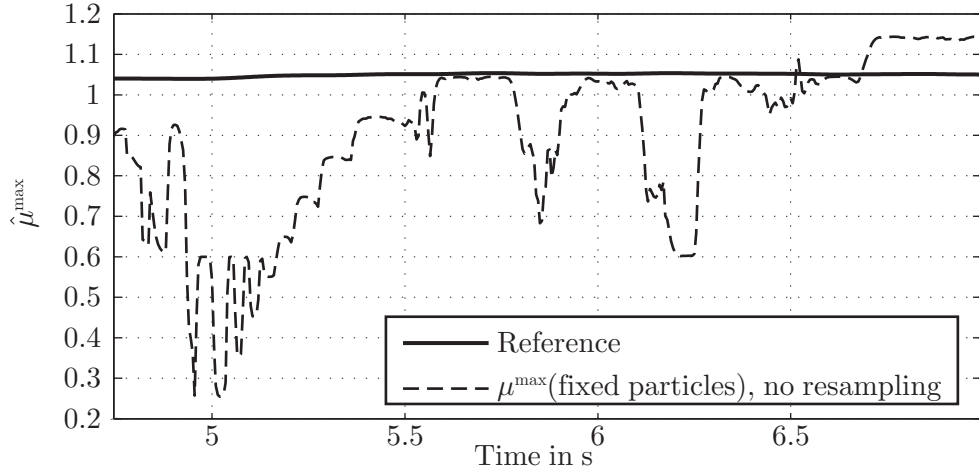
Figure 6.3.: Estimate of \mu^{\max} for a driving manoeuvre with a longitudinal acceleration of b a_x \approx 4.5 \text{ m/s}^2 with fixed particles of \mu^{\max} for all time steps. The mean absolute error (MAE) of the estimate is 0.1725 and the maximum absolute error of 0.7860 occurs around second 5, see also Table 6.1.
